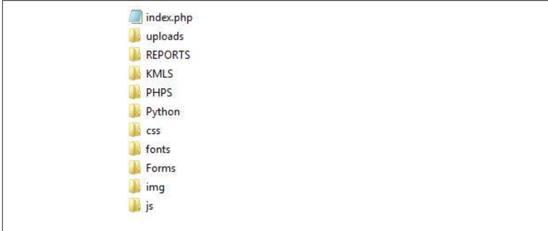
Figure 0.1: application folders.
