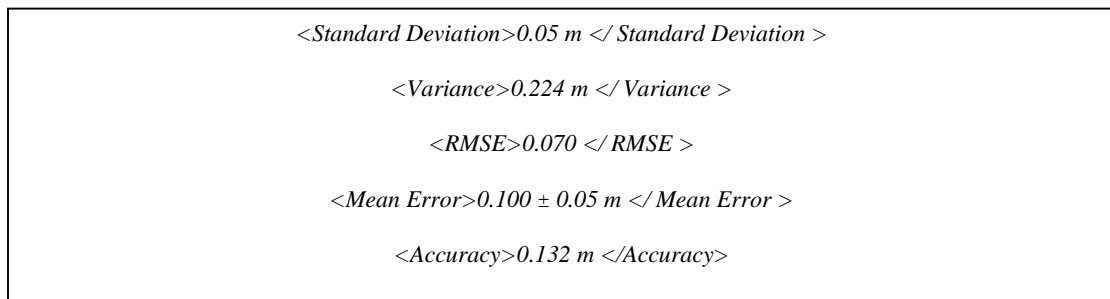
Figure 0.12: This figure shows the proposed report schema after a DEM or TIN has been evaluated.
