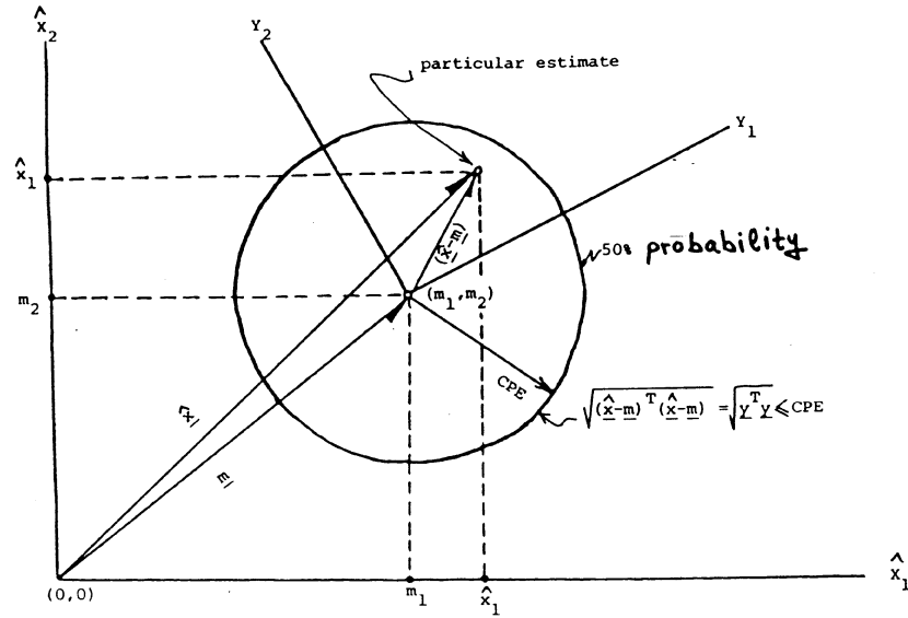
Figure 3.7: Geometrical Depiction of the CPE Circle.
