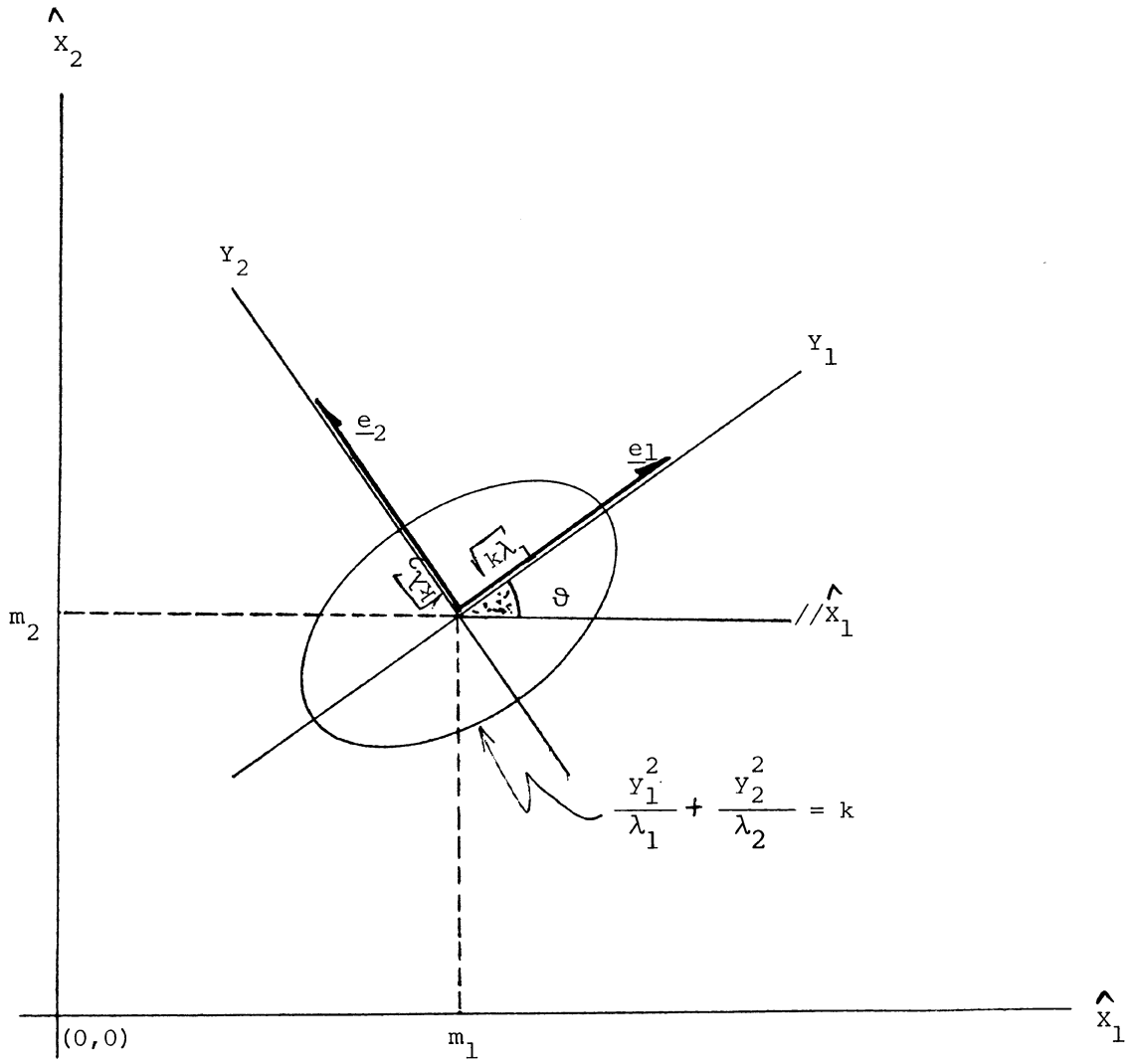
Figure 3.3: Confidence Ellipse (u=2)
