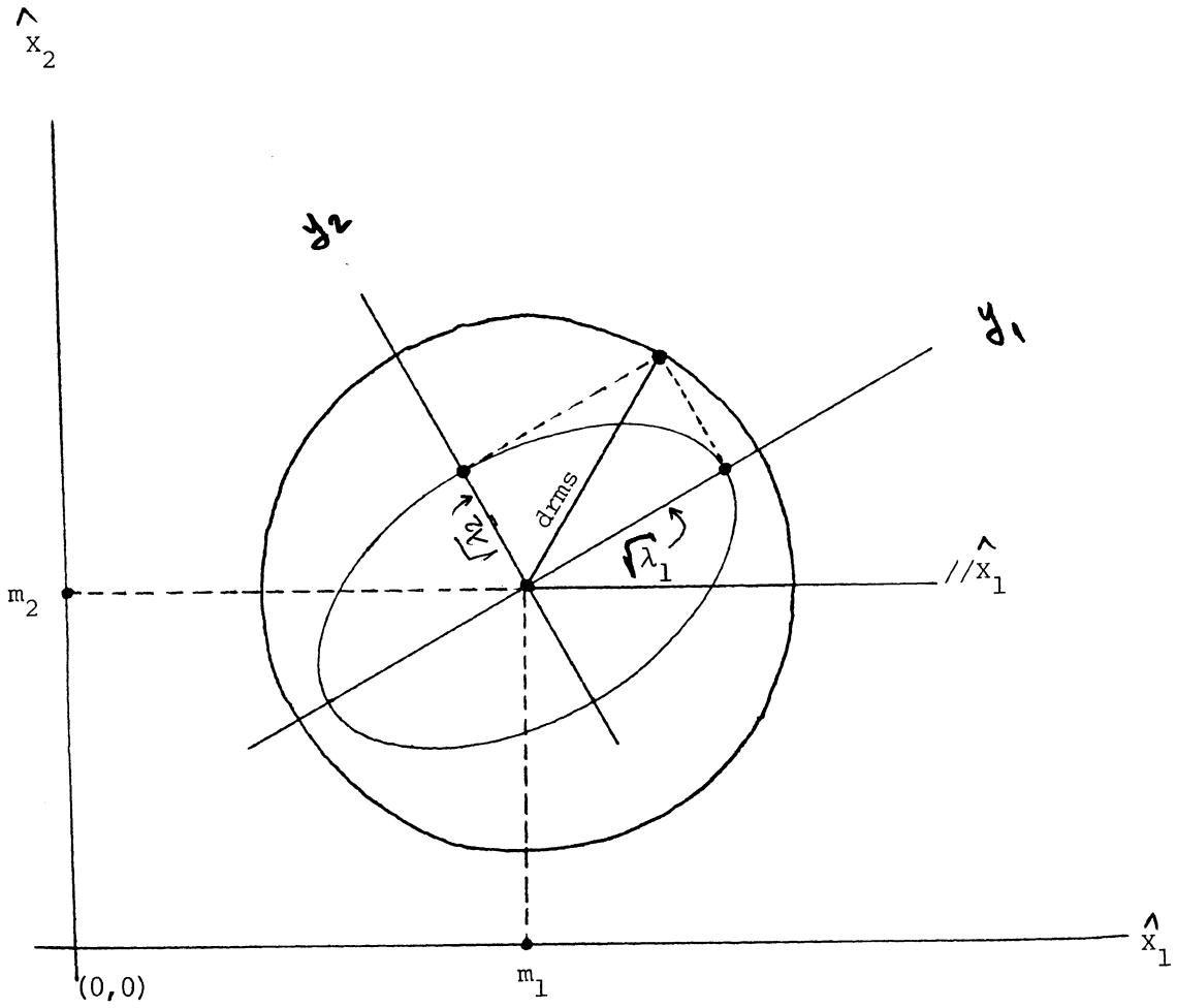
Figure 3.13: The drms Radial Error ( \text{drms} = \sqrt{\sigma_1^2 + \sigma_2^2} = \sqrt{\lambda_1 + \lambda_2} )
