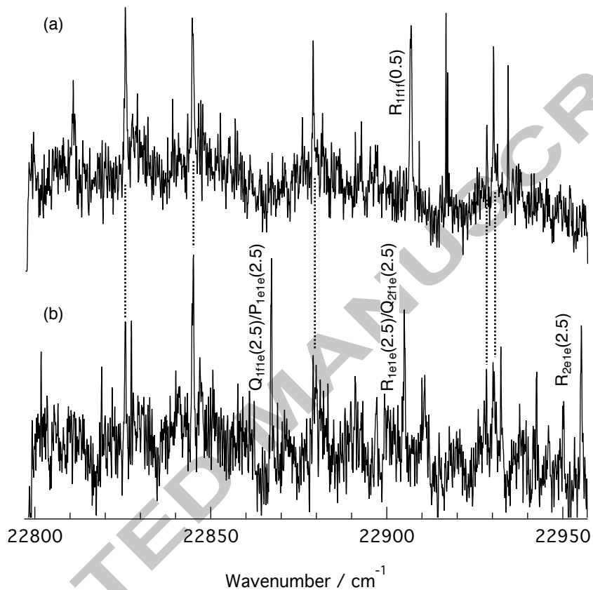
Figure 3: Two-photon scans of the 1\ ^2\Delta - A\ ^2\Pi 0-0 band of MgH. One laser is fixed and populates a particular rotational level of the A\ ^2\Pi state via the A\ ^2\Pi - X\ ^2\Sigma^+ transition, and a second laser is scanned to excite all possible levels of the 1\ ^2\Delta - A\ ^2\Pi transition accessible from the pumped level. The spectra shown are taken in laser-induced fluorescence as a function of wavenumber of the second laser beam. Spectrum (a) arose from excitation of the A\ ^2\Pi\ F_1\ J = 0.5\ f level with the pumping laser beam, from which only the one labelled 1\ ^2\Delta - A\ ^2\Pi transition was possible. For spectrum (b) the F_1\ J = 2.5\ e level was pumped, and three transitions (two of which are unresolved doublets) were seen and are labelled. Dotted lines mark examples of lines from unknown species which appear regardless of whether the A\ ^2\Pi pump laser is blocked or released.
