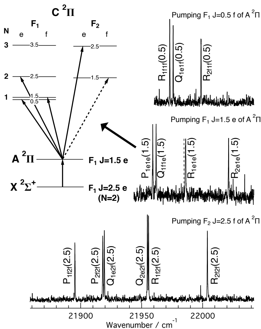
Figure 2: Two-photon scans of the C^2\Pi - A^2\Pi 0-0 band of MgH. One laser is fixed and populates a particular rotational level of the A^2\Pi state via the A^2\Pi - X^2\Sigma^+ transition, and a second laser excites all possible levels of the C^2\Pi - A^2\Pi transition accessible from the pumped level. The spectra shown are taken in laser-induced fluorescence as a function of wavenumber of the second laser beam. The energy levels and transitions corresponding to the middle spectrum are shown in the inset. The dotted lines in the middle spectrum and energy diagram indicate a transition that was expected, but did not appear (see the text).
